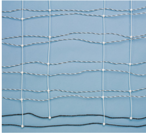
Premier ElectroNet™ Product #: C26081
